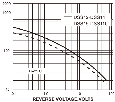
FIG. 5-TYPICAL JUNCTION CAPACITANCE
