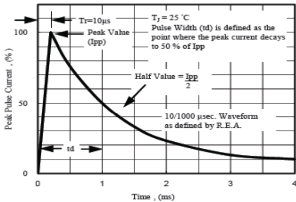
Fig. 5 - Pulse Waveform
